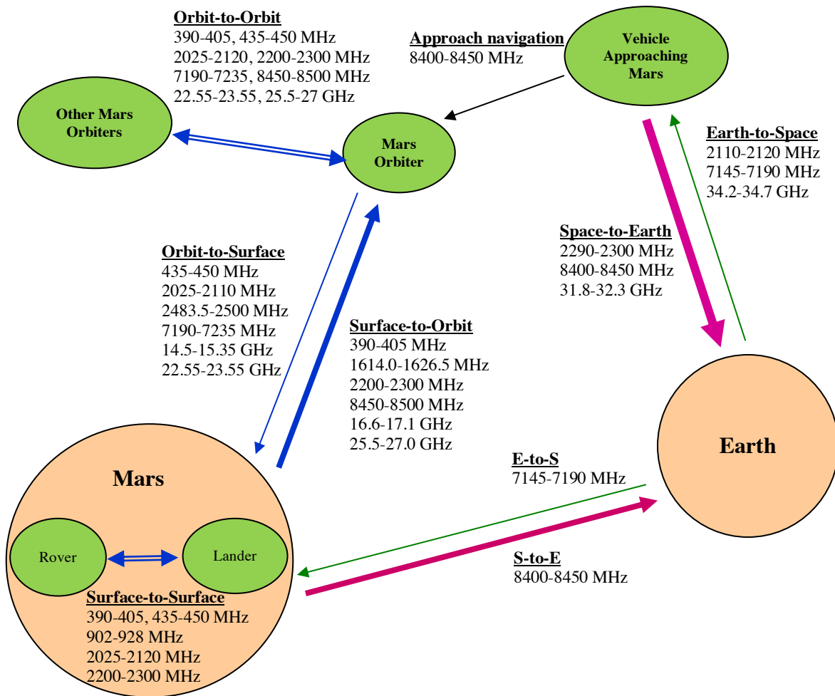
Figure 1. Conceptual Mars Communications Frequency Scenario
